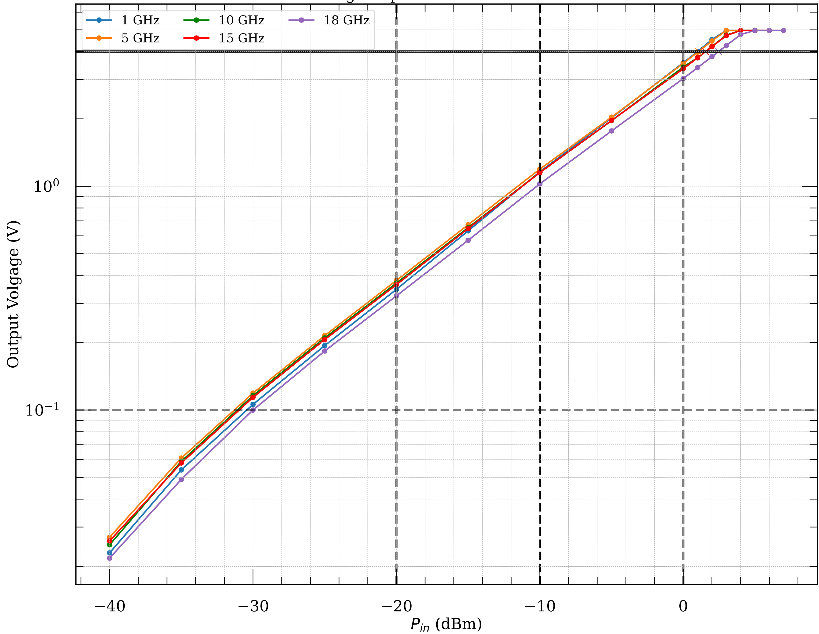
Measured voltage-to-power curve of detector module038
